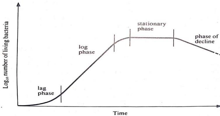
Fig 2.15 Typical growth curve of a bacterial population.
